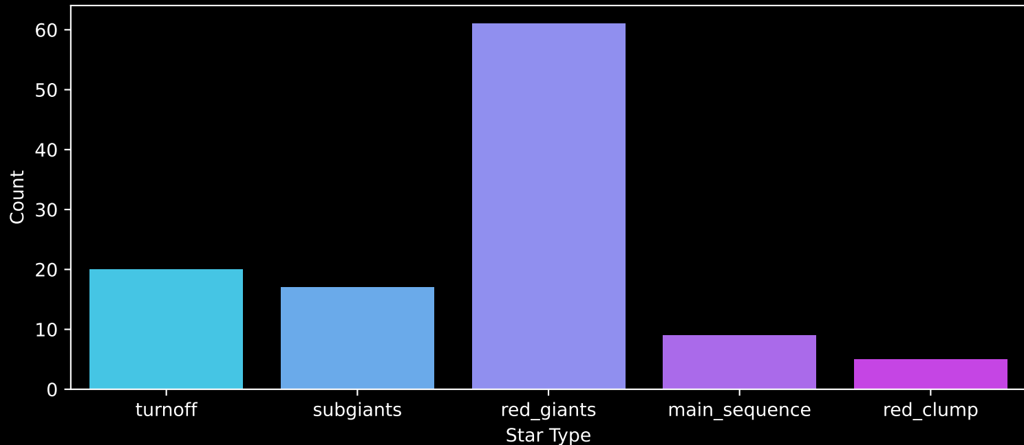
APOGEE DR17 Field: [008+00] Count plot of Star Type
