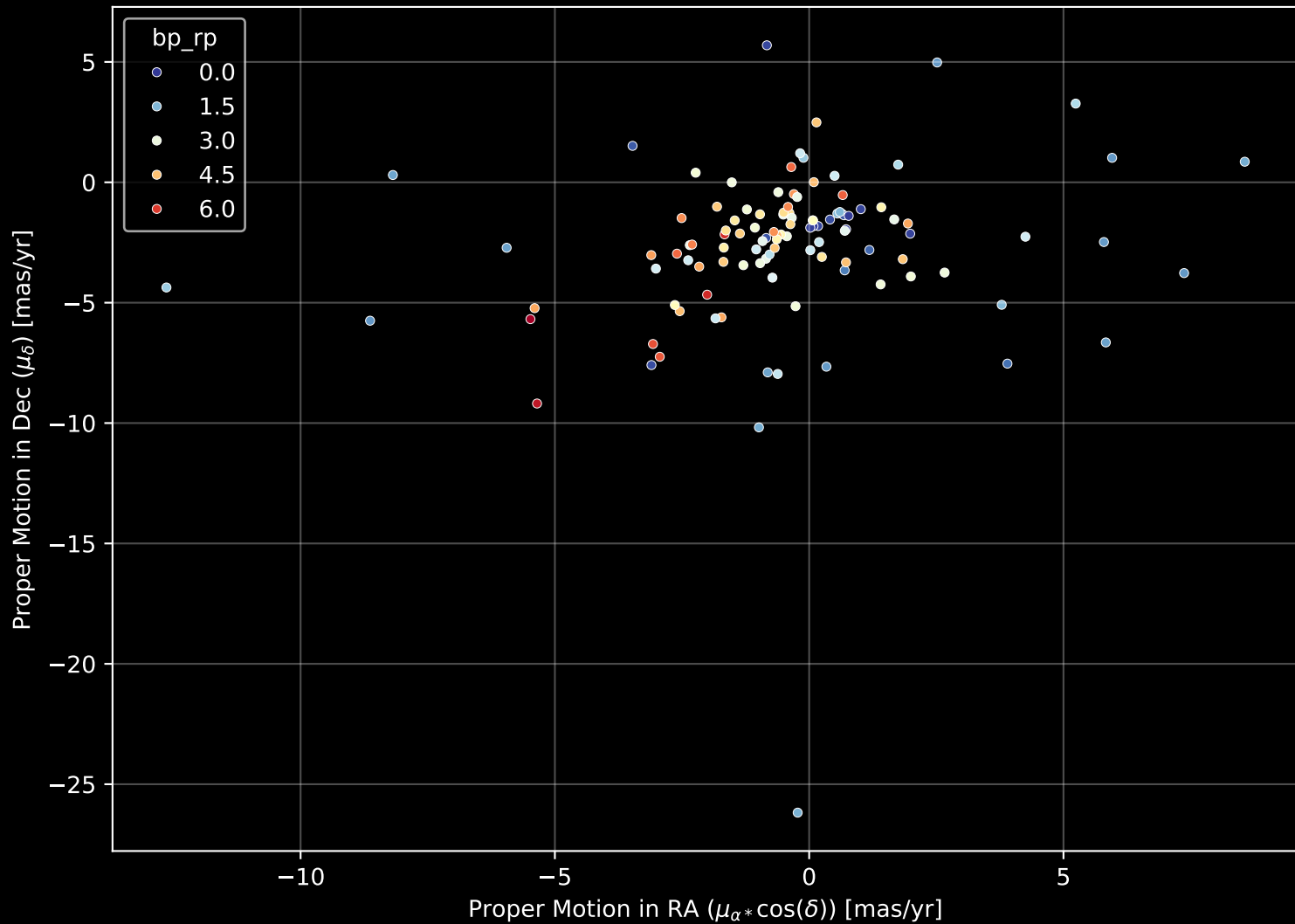
APOGEE DR17 Field: [008+00] Proper Motion Diagram (n= 112)
