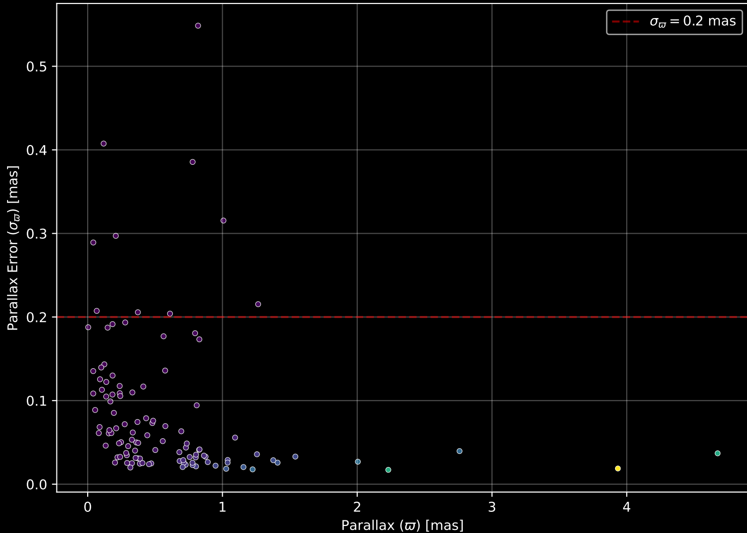
APOGEE DR17 Field: [008+00] Parallax Quality (n= 112)
