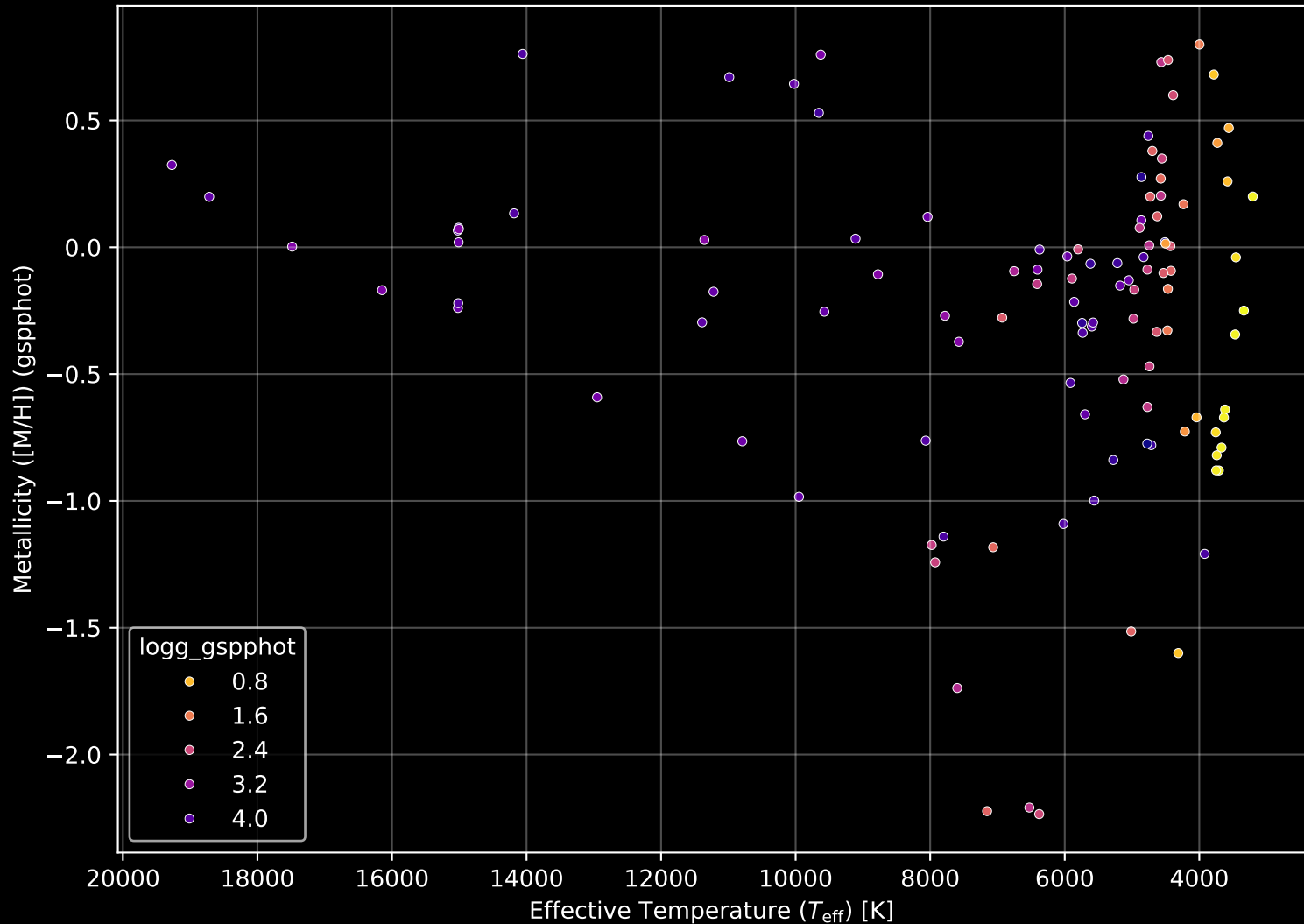
APOGEE DR17 Field: [008+00] Stellar Population Parameters (n= 112)
