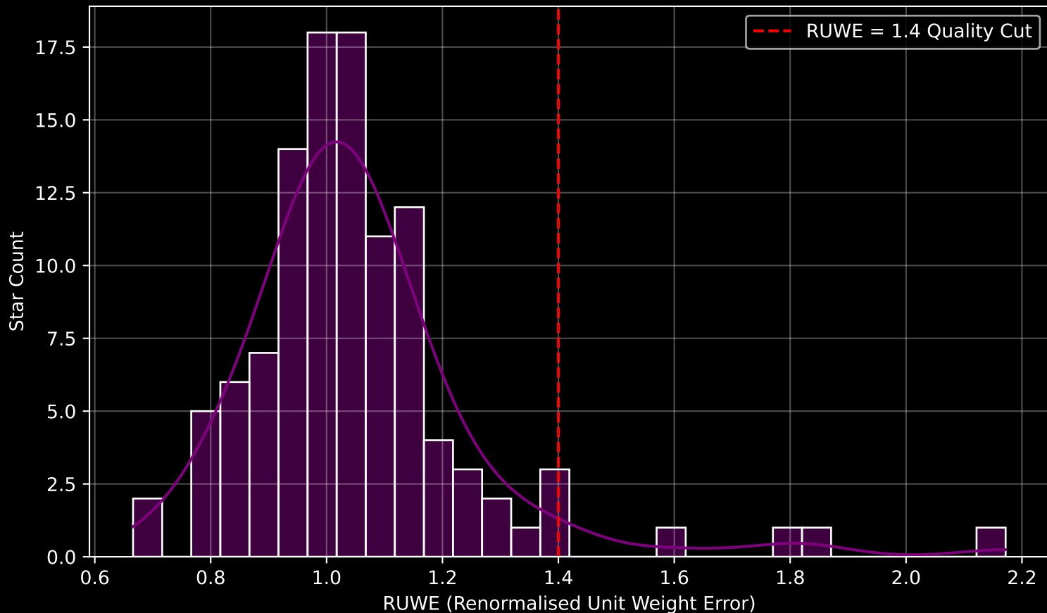
GAPOGEE DR17 Field [008+00] RUWE Distribution (n= 110)
