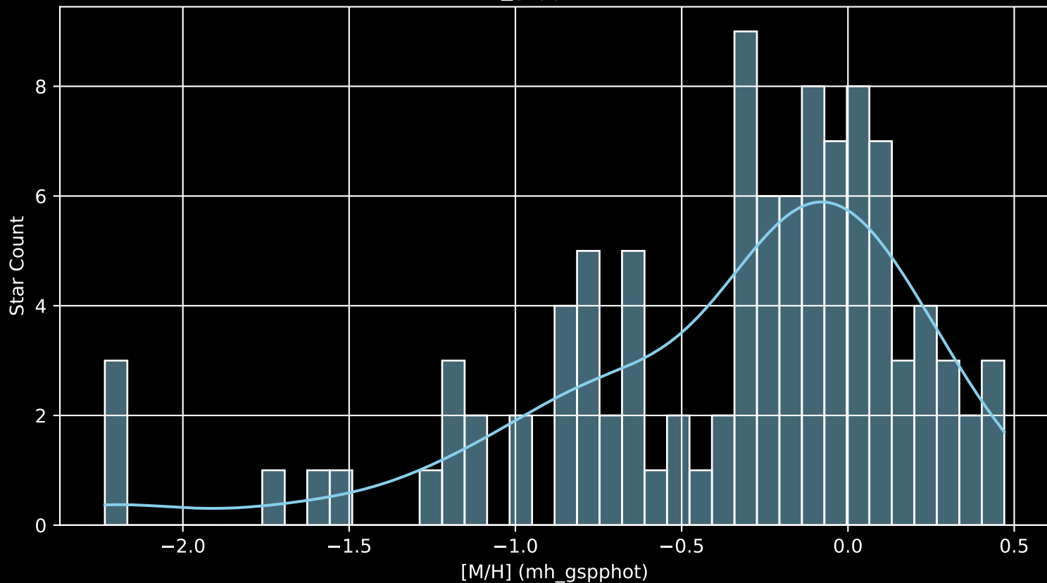
APOGEE DR17 Field: [008+00 [M/H] (mh_gspphot) (n= 102)
